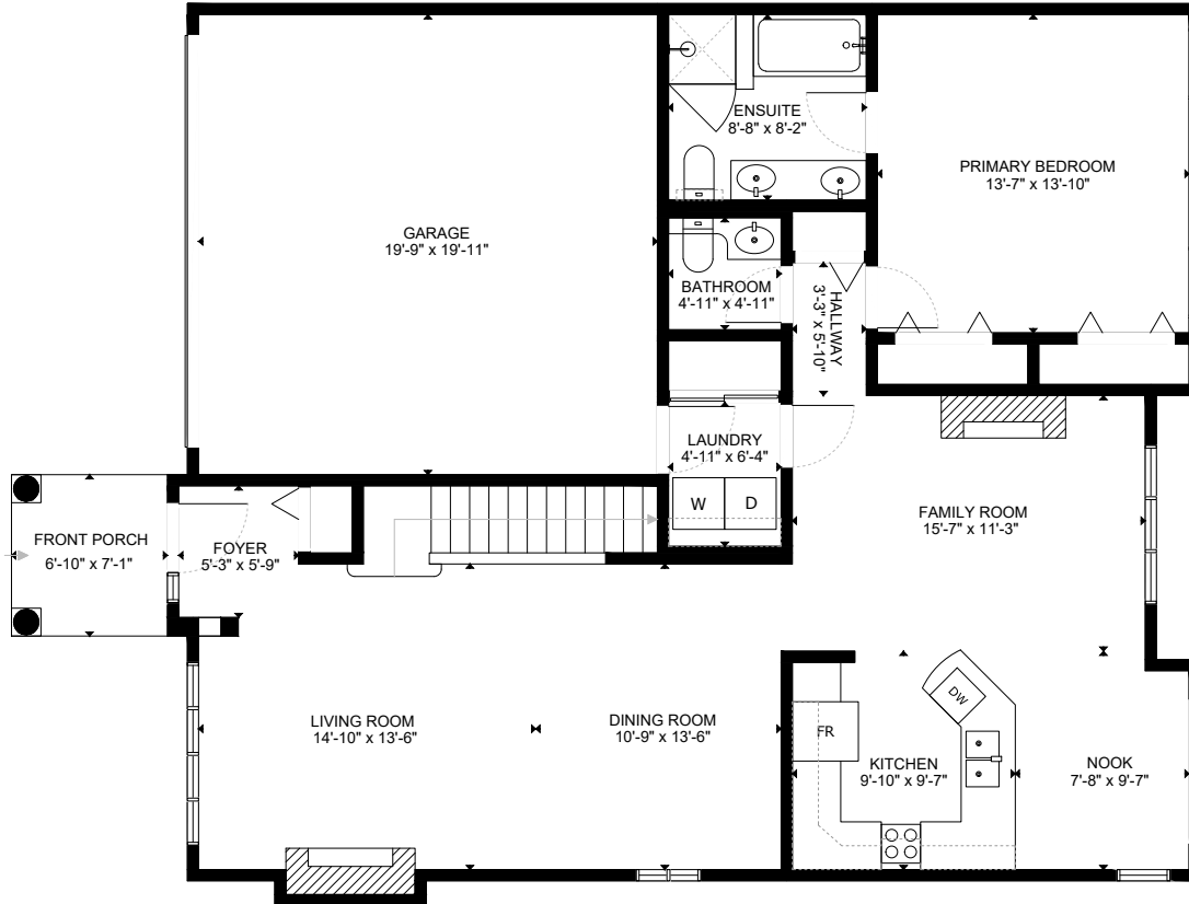
MAIN FLOOR 1285 sq ft CEILING HEIGHT: 18'-2"
